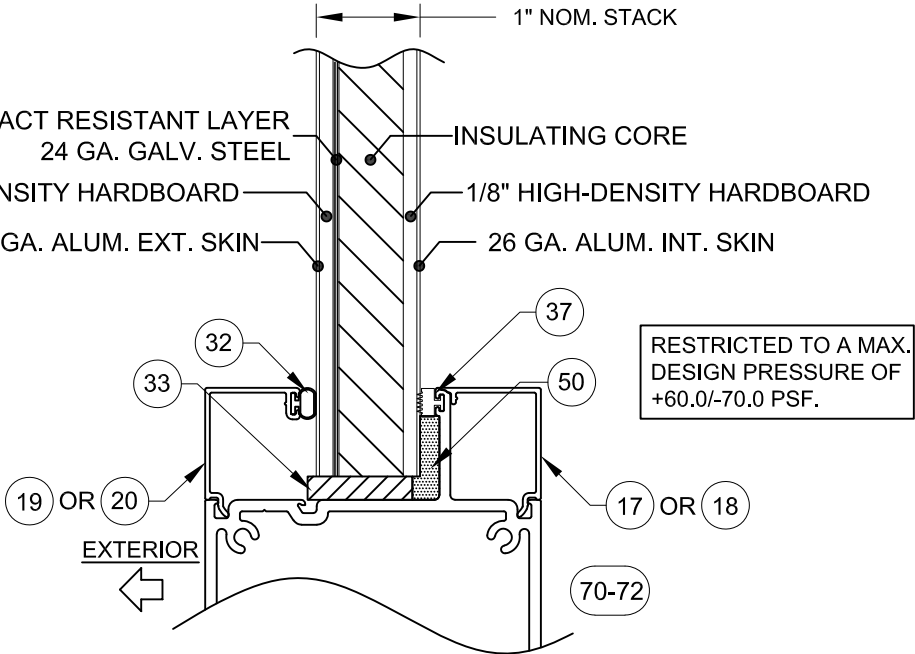
OPAQUE PANEL
