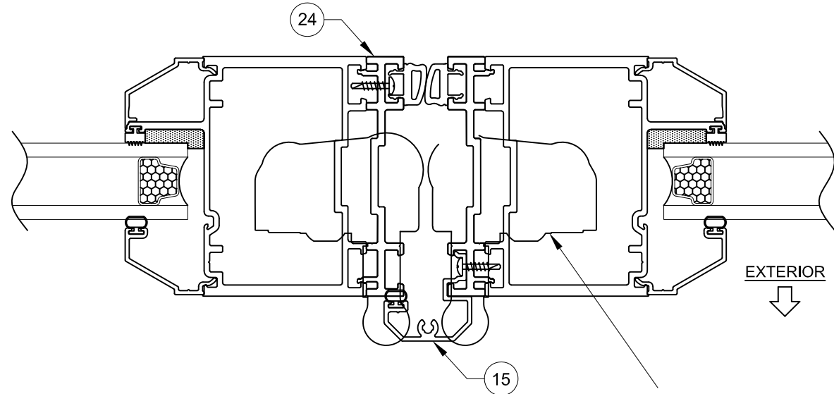
DETAIL K
