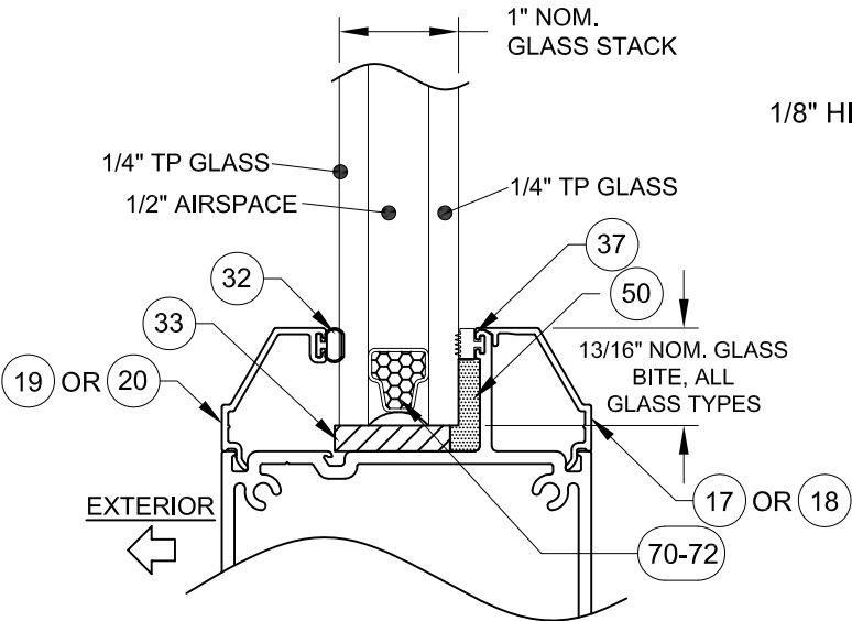
GLASS TYPE 2
