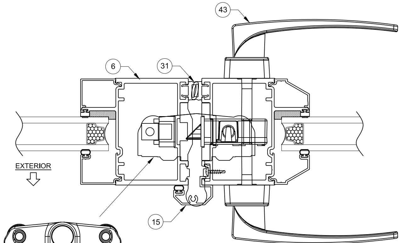
DETAIL E
