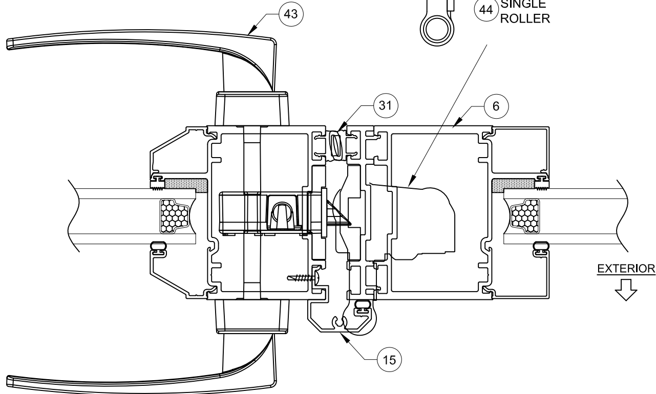
DETAIL L
